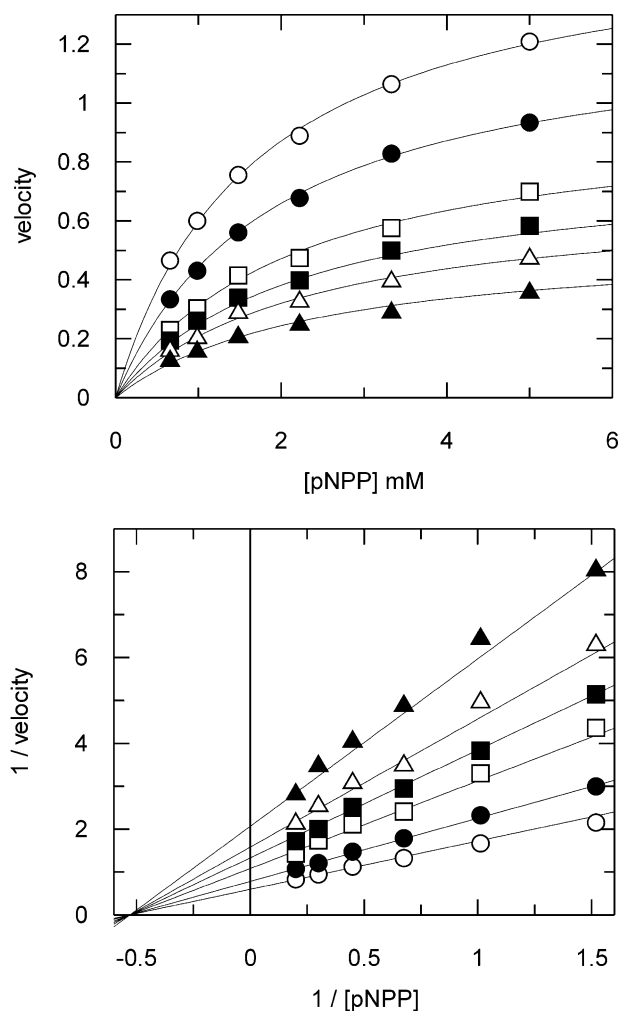
Figure 1. Compound 11 behaves as a non-competitive inhibitor or PTP1B. Top panel: velocity curves performed with 20 ng PTP1B in the presence of increasing concentrations of compound 11 (open circles, 0 μM, filled circles, 1.25 μM, open squares, 3.3 μM, filled squares, 5 μM, open triangles, 6.7 μM, filled triangles, 10 μM). Data are representative of several experiments, each point the average of quadruplicates. Solid lines are fits of the data to the Henri Michaelis Menten equation. Lower panel: Lineweaver–Burke transformations of data from top panel.
