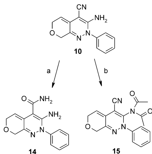
Scheme 2. Reagents: (a) concd \text{H}_2\text{SO}_4 , 80\text{--}90^\circ\text{C} ; (b) \text{Ac}_2\text{O} , Hunigs base, \text{CH}_2\text{Cl}_2 .
