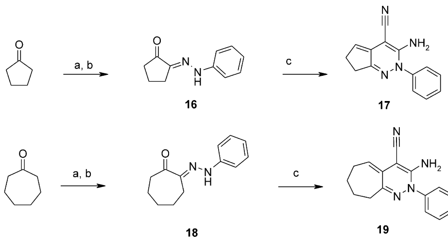
Scheme 3. Reagents: (a) \text{NaH} , \text{HCO}_2\text{Et} , \text{EtOH} ; (b) \text{PhN}_2^+\text{Cl}^- , -5^\circ\text{C} ; (c) malononitrile, morpholine, DMSO.
